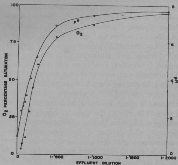
Fig. 1—Changes in pH and oxygen percentage saturation at different dilutions of the effluent
