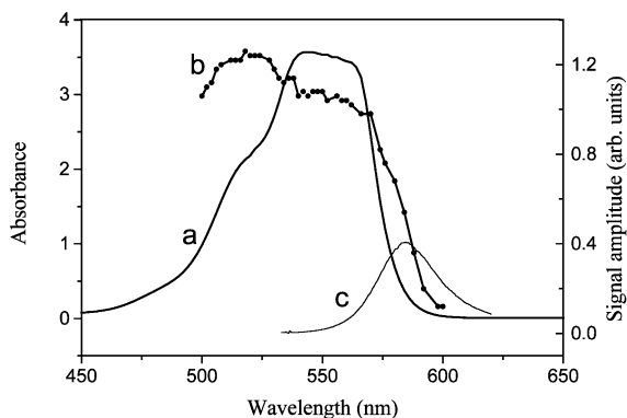
Fig. 3. Spectra of rhodamine B for a concentration of 460 \mu\text{mol l}^{-1} in methanol (a) absorption spectrum (b) thermal lens spectrum (c) fluorescence spectrum.
