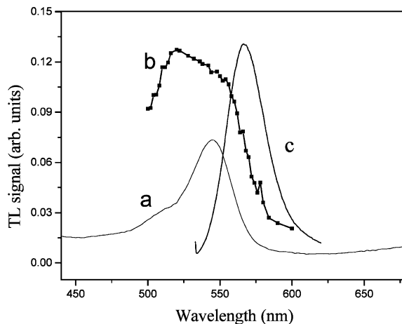
Fig. 2. Spectra of rhodamine B for a concentration of 2.68 μmol l -1 in methanol (a) absorption spectrum (b) thermal lens spectrum (c) fluorescence spectrum.
