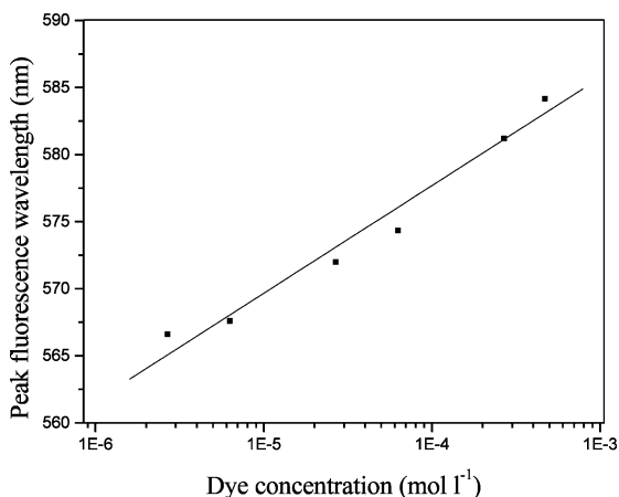
Fig. 4. The concentration dependence of peak fluorescence wavelength of rhodamine B.
